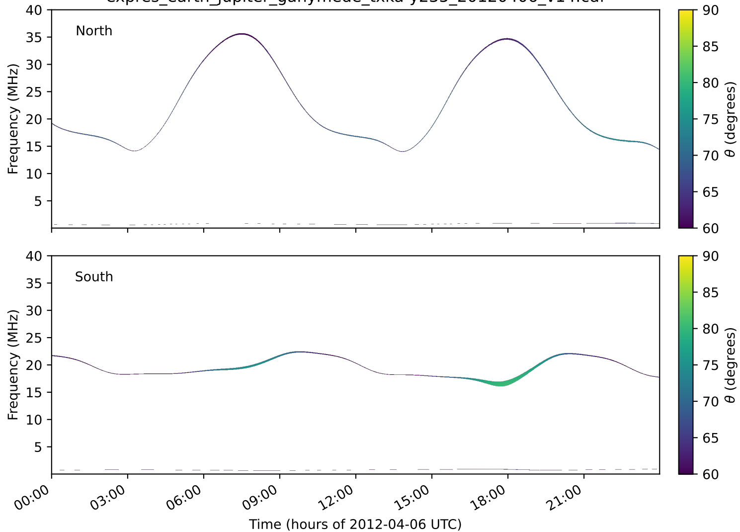
expres_earth_jupiter_ganymede_txka-y235_20120406_v14.cdf
