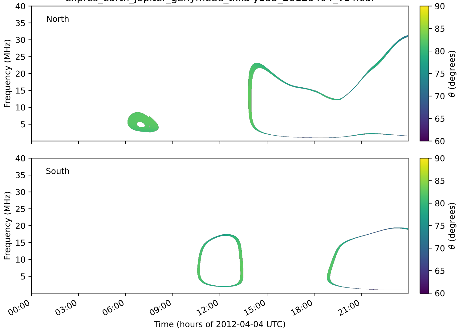
expres_earth_jupiter_ganymede_txka-y235_20120404_v14.cdf
