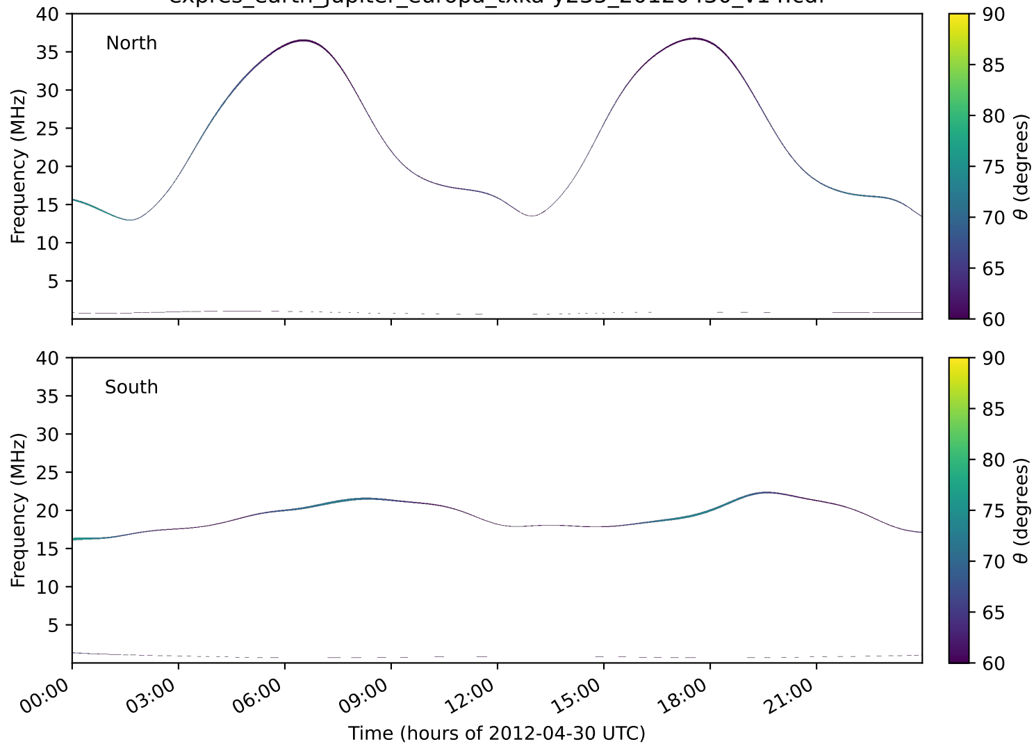
expres_earth_jupiter_europa_txka-y235_20120430_v14.cdf
