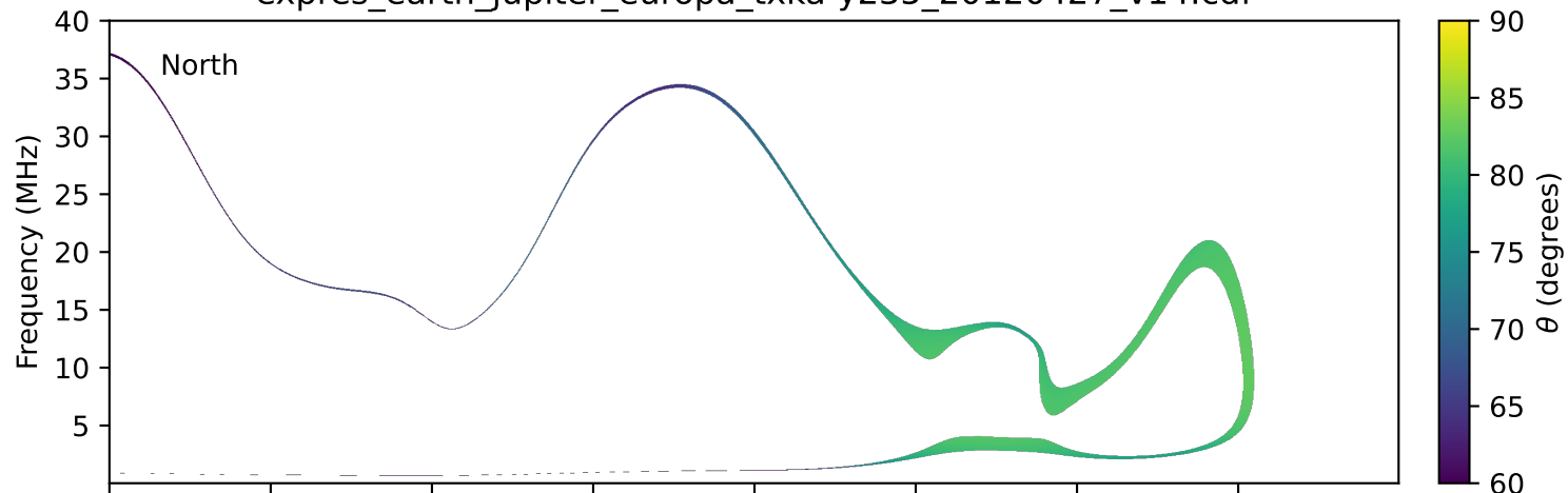
expres_earth_jupiter_europa_txka-y235_20120427_v14.cdf
