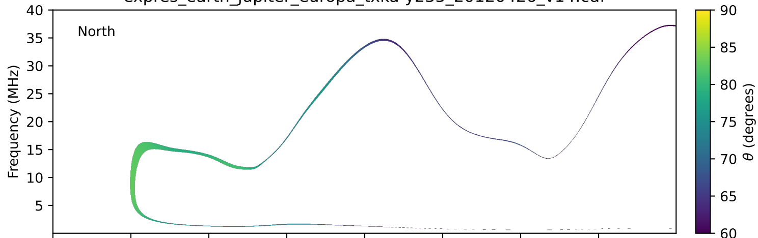
expres_earth_jupiter_europa_txka-y235_20120426_v14.cdf
