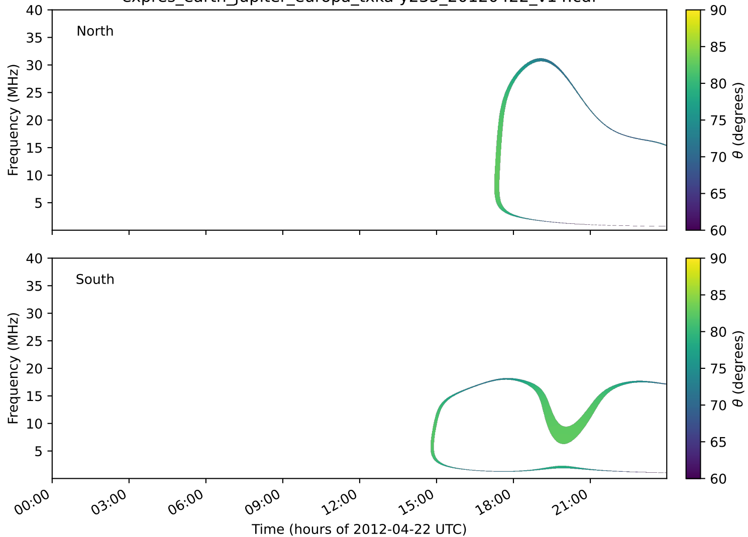
expres_earth_jupiter_europa_txka-y235_20120422_v14.cdf
