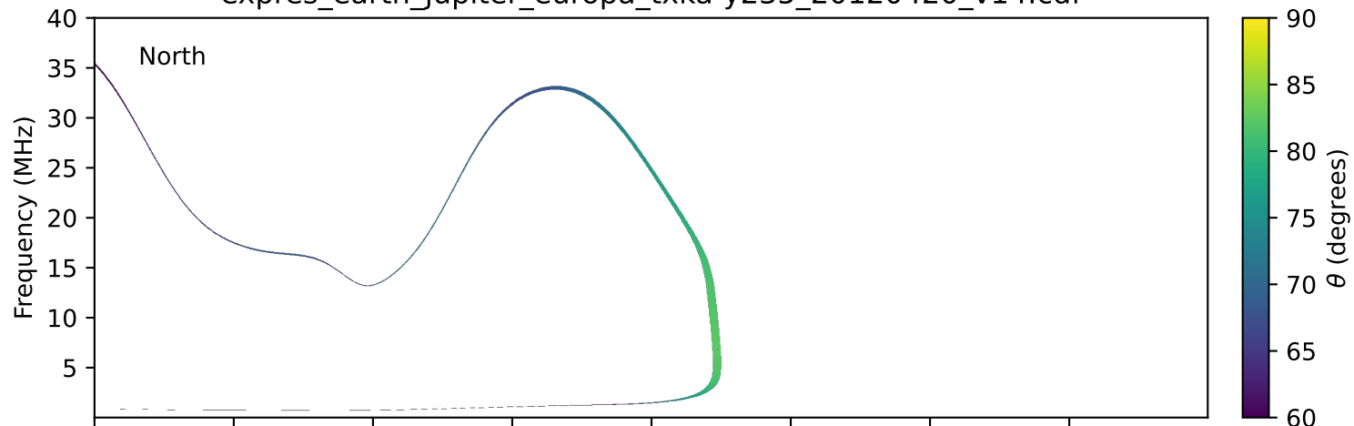
expres_earth_jupiter_europa_txka-y235_20120420_v14.cdf
