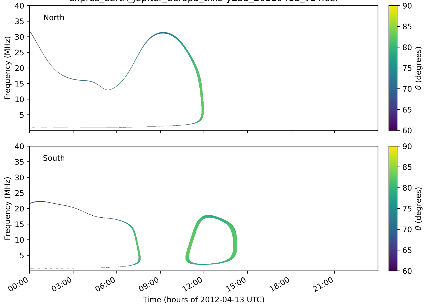
expres_earth_jupiter_europa_txka-y235_20120413_v14.cdf
