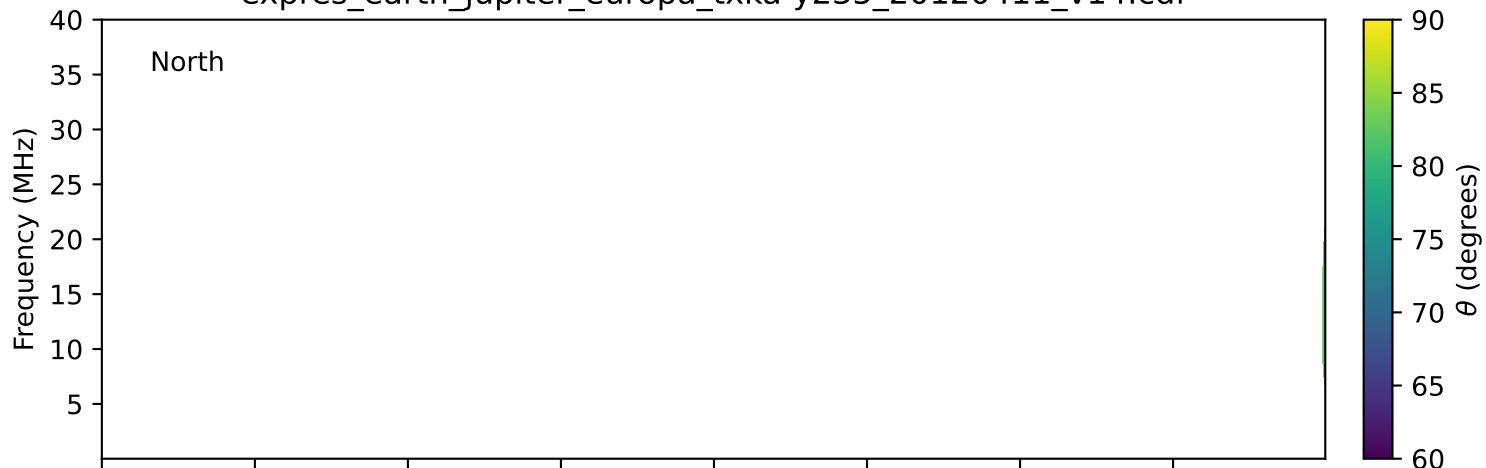
expres_earth_jupiter_europa_txka-y235_20120411_v14.cdf
