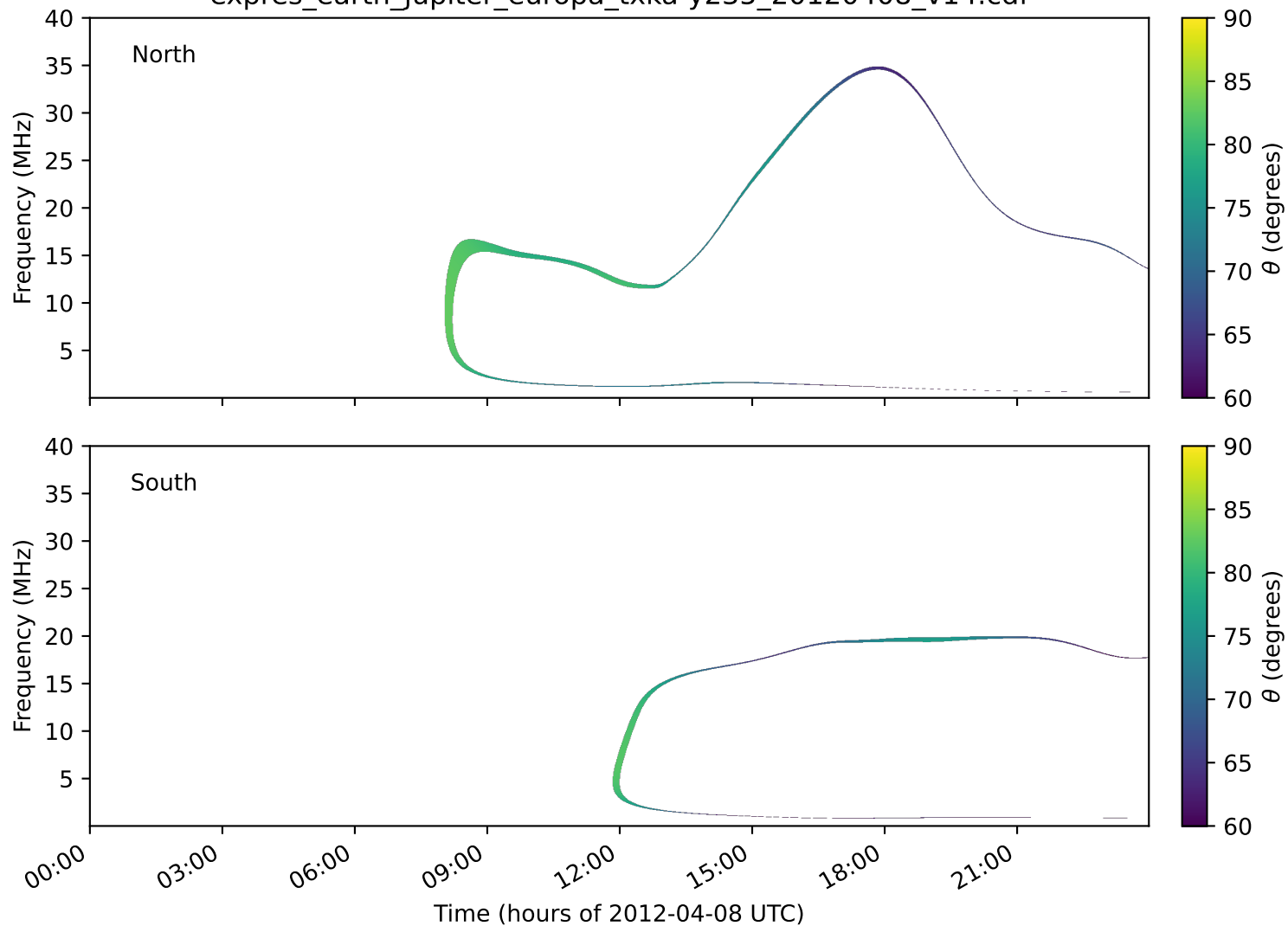
expres_earth_jupiter_europa_txka-y235_20120408_v14.cdf
