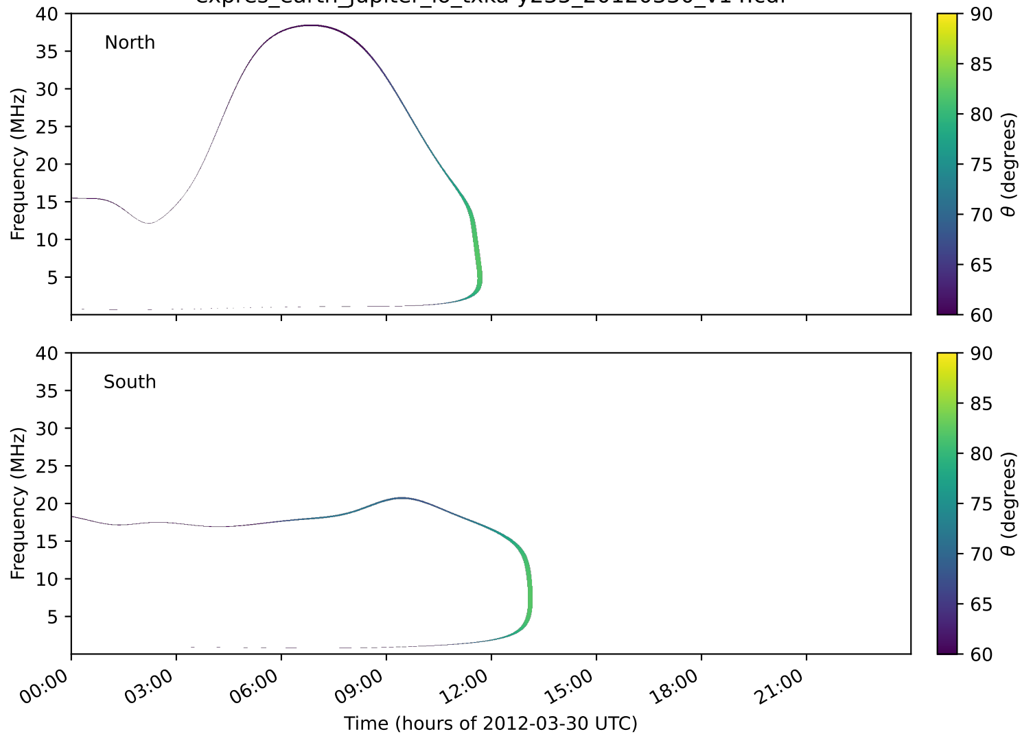
expres_earth_jupiter_io_txka-y235_20120330_v14.cdf
