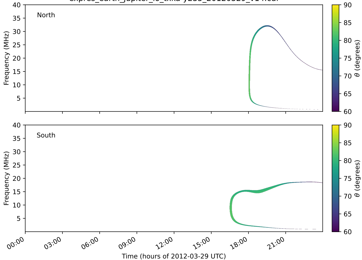
expres_earth_jupiter_io_txka-y235_20120329_v14.cdf
