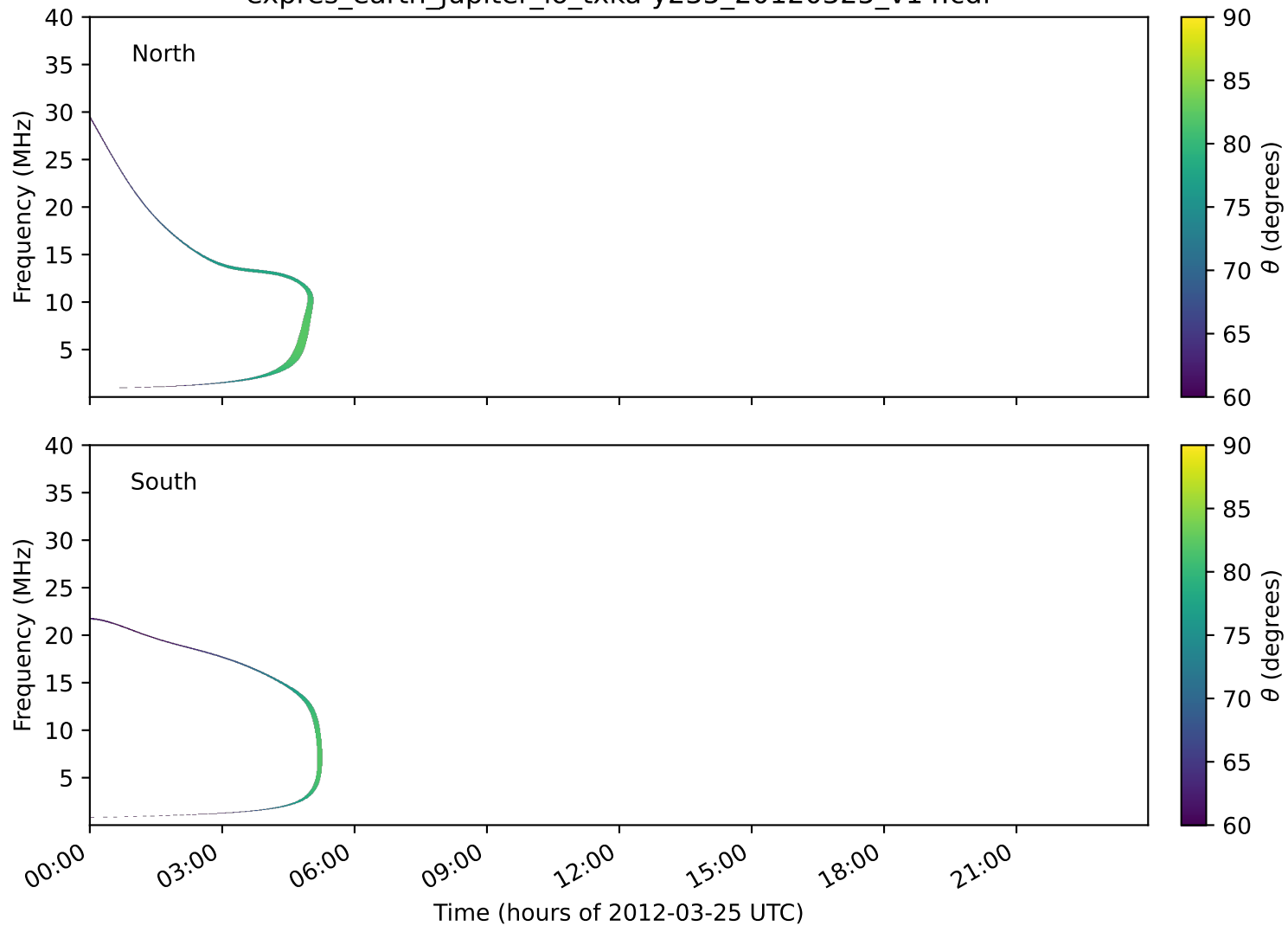
expres_earth_jupiter_io_txka-y235_20120325_v14.cdf
