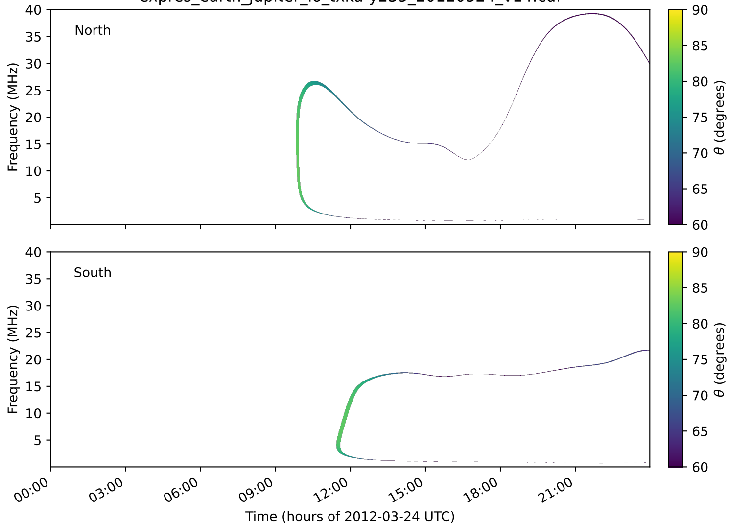
expres_earth_jupiter_io_txka-y235_20120324_v14.cdf
