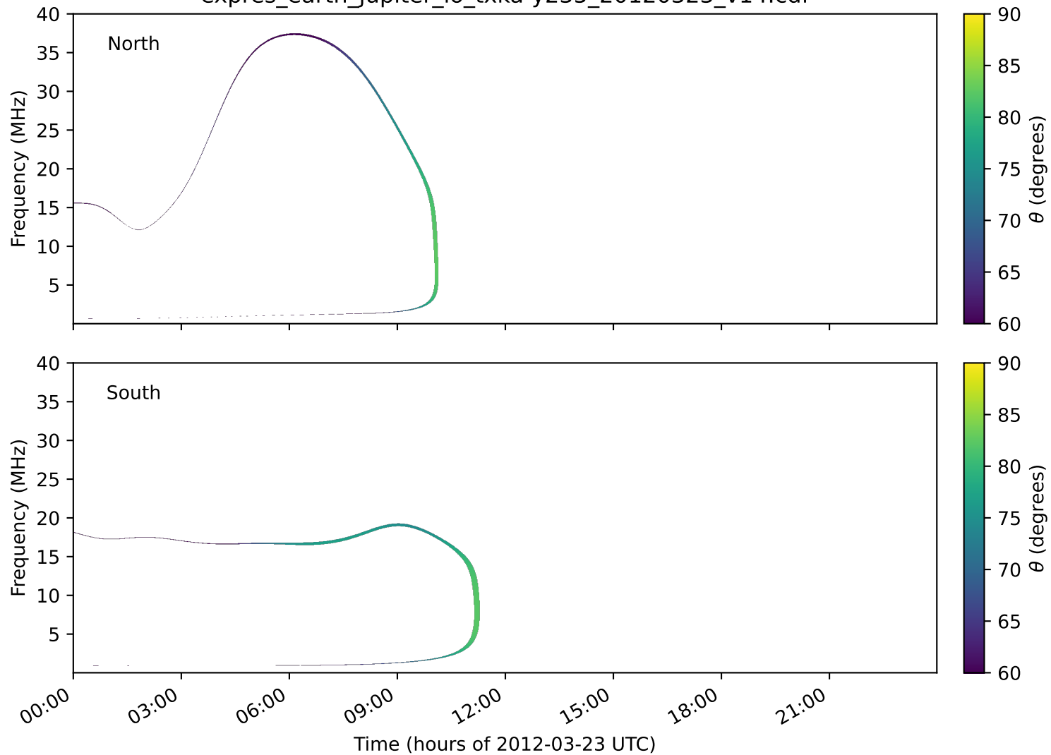
expres_earth_jupiter_io_txka-y235_20120323_v14.cdf
