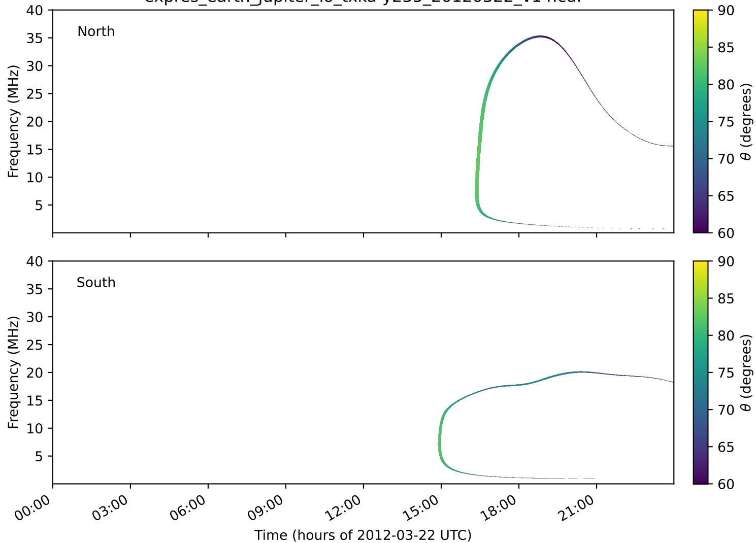
expres_earth_jupiter_io_txka-y235_20120322_v14.cdf
