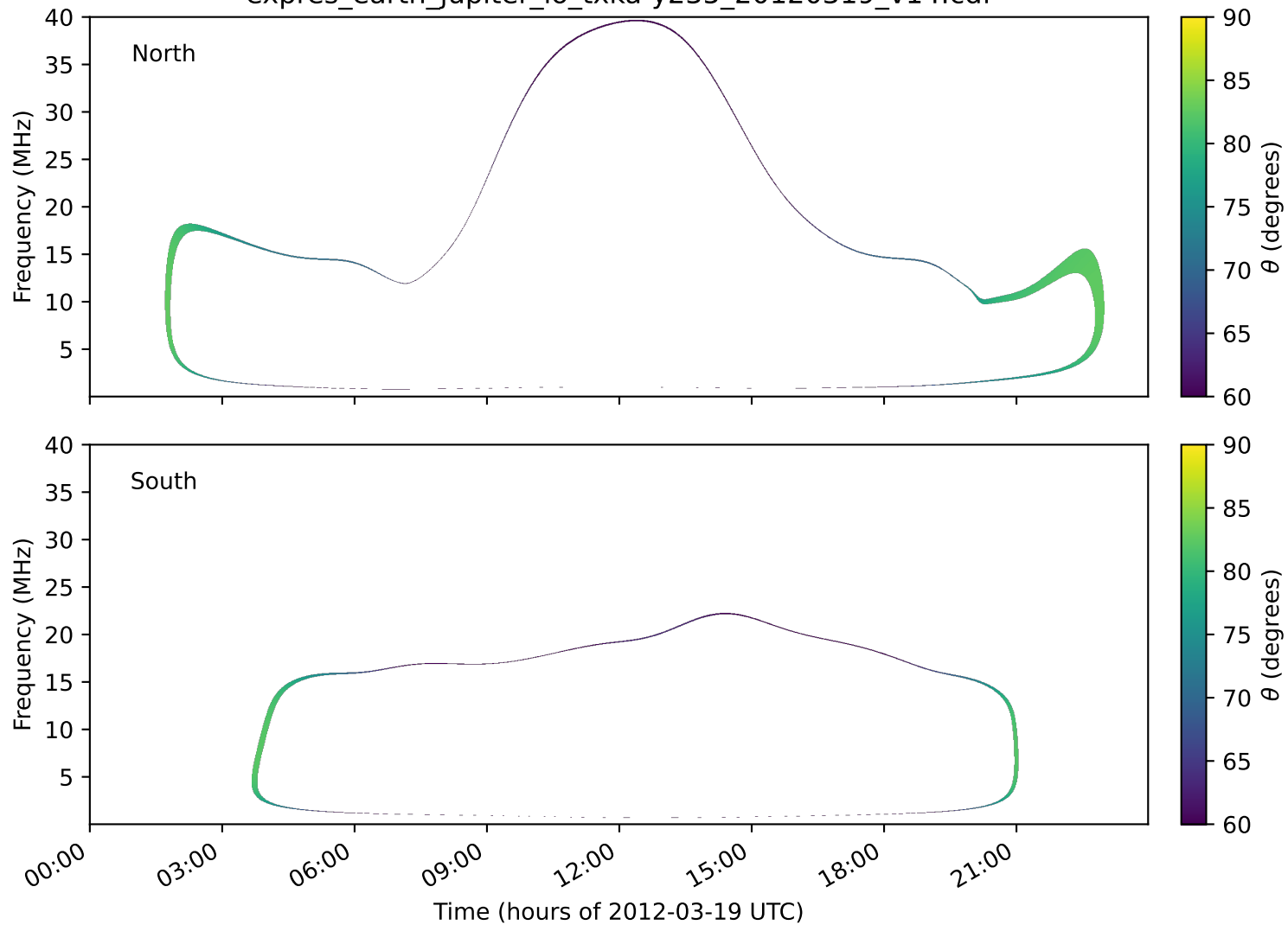
expres_earth_jupiter_io_txka-y235_20120319_v14.cdf
