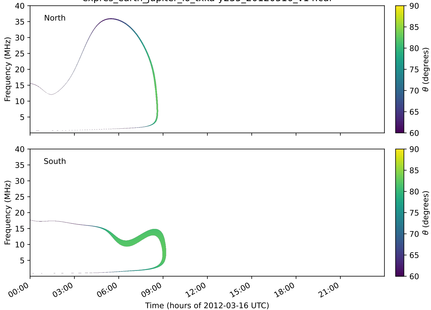
expres_earth_jupiter_io_txka-y235_20120316_v14.cdf
