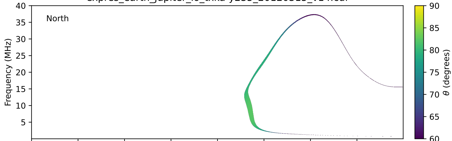
expres_earth_jupiter_io_txka-y235_20120315_v14.cdf
