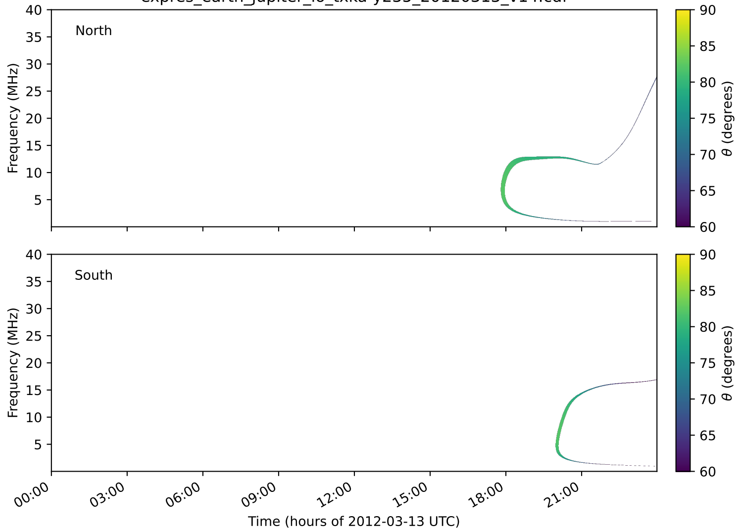
expres_earth_jupiter_io_txka-y235_20120313_v14.cdf
