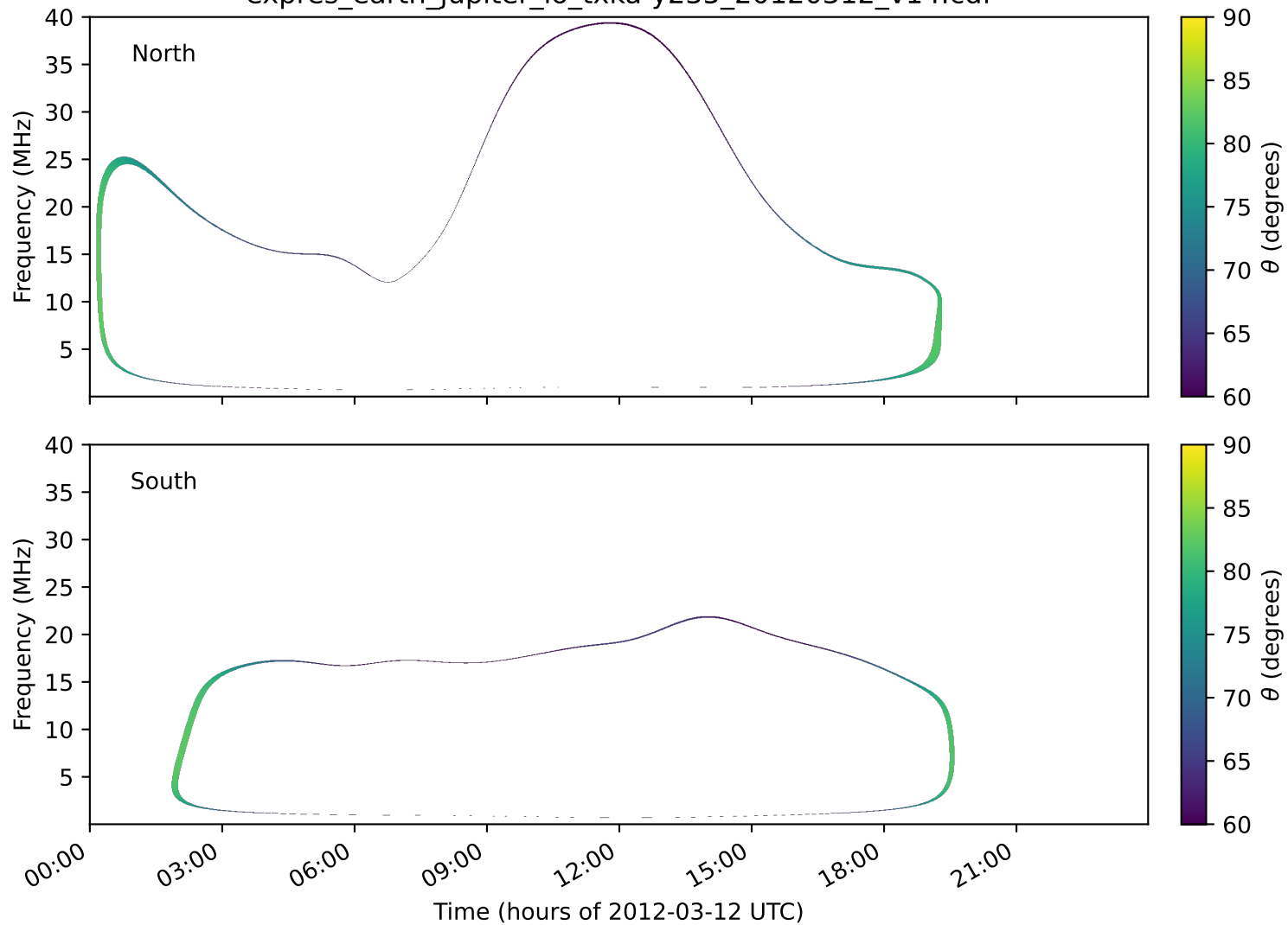
expres_earth_jupiter_io_txka-y235_20120312_v14.cdf
