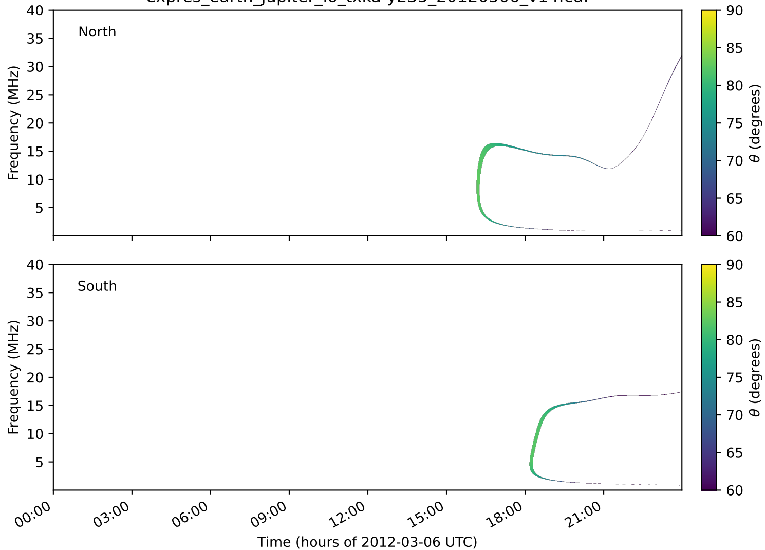
expres_earth_jupiter_io_txka-y235_20120306_v14.cdf
