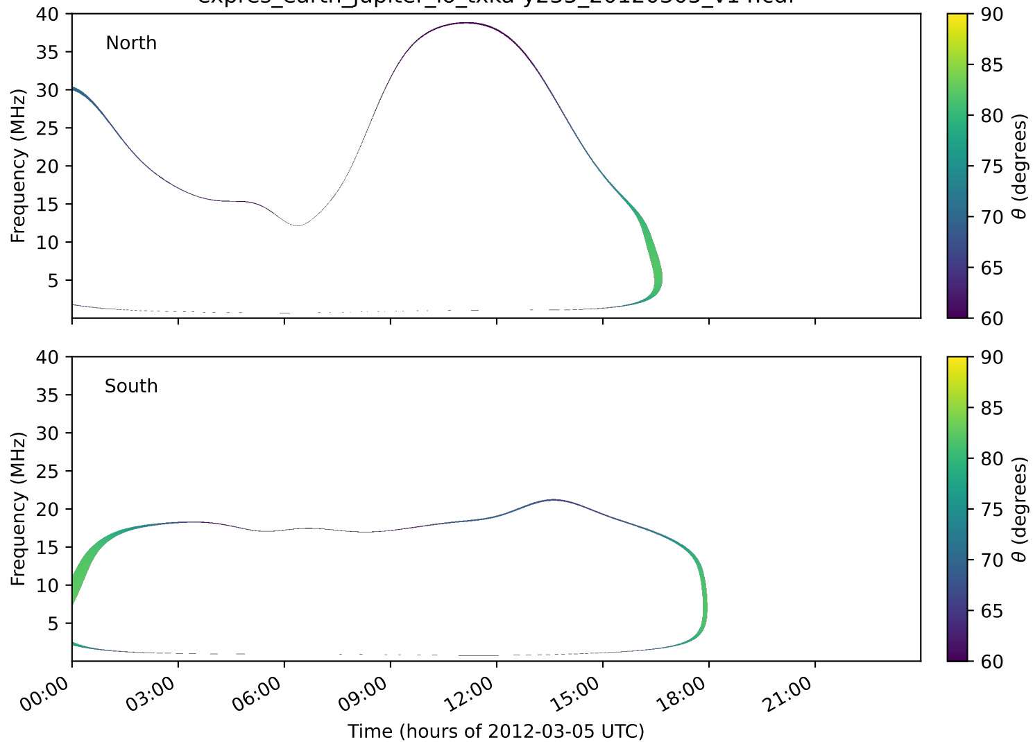
expres_earth_jupiter_io_txka-y235_20120305_v14.cdf
