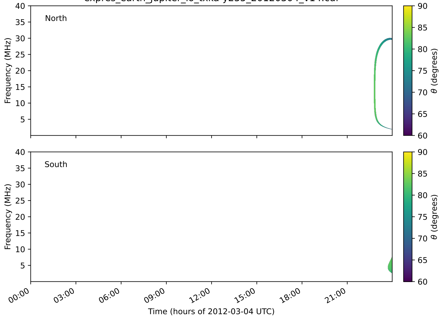
expres_earth_jupiter_io_txka-y235_20120304_v14.cdf
