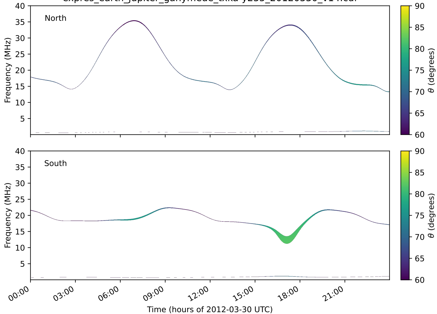
expres_earth_jupiter_ganymede_txka-y235_20120330_v14.cdf
