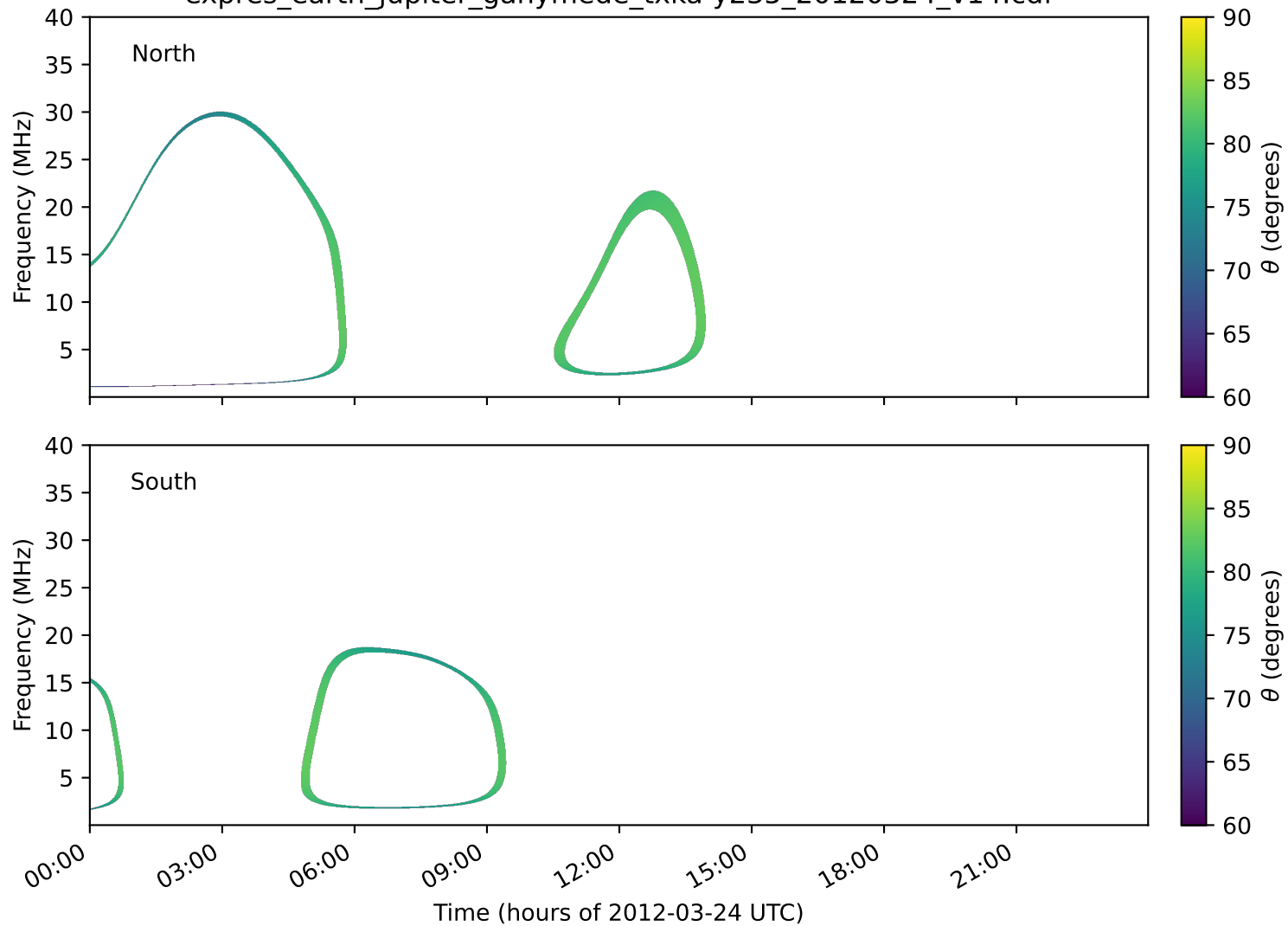
expres_earth_jupiter_ganymede_txka-y235_20120324_v14.cdf
