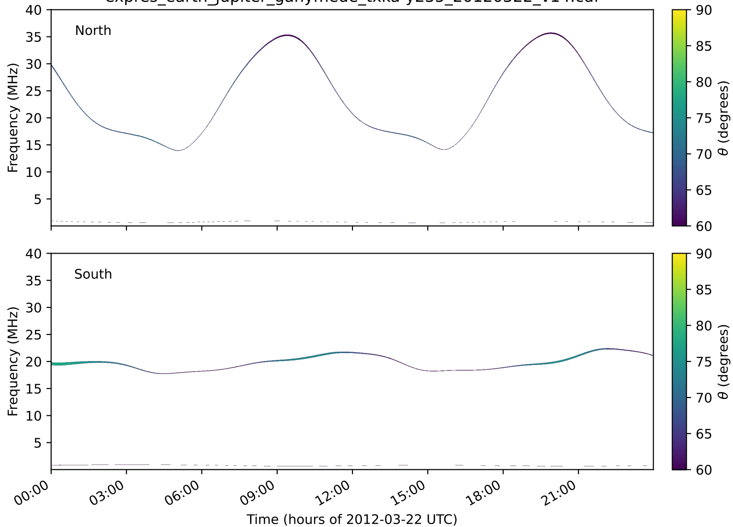
expres_earth_jupiter_ganymede_txka-y235_20120322_v14.cdf
