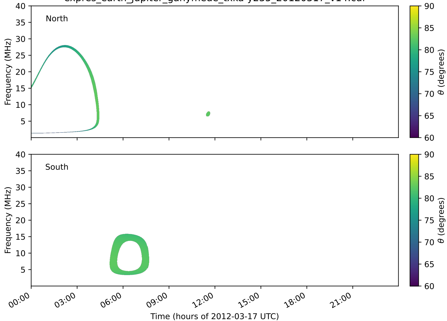
expres_earth_jupiter_ganymede_txka-y235_20120317_v14.cdf
