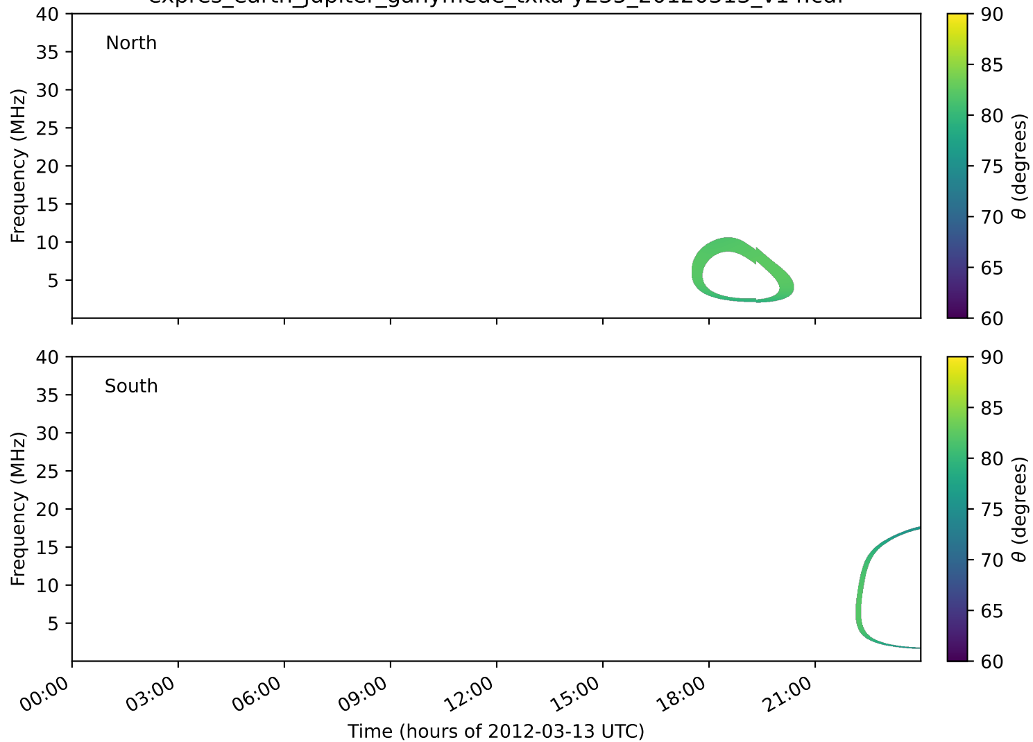
expres_earth_jupiter_ganymede_txka-y235_20120313_v14.cdf
