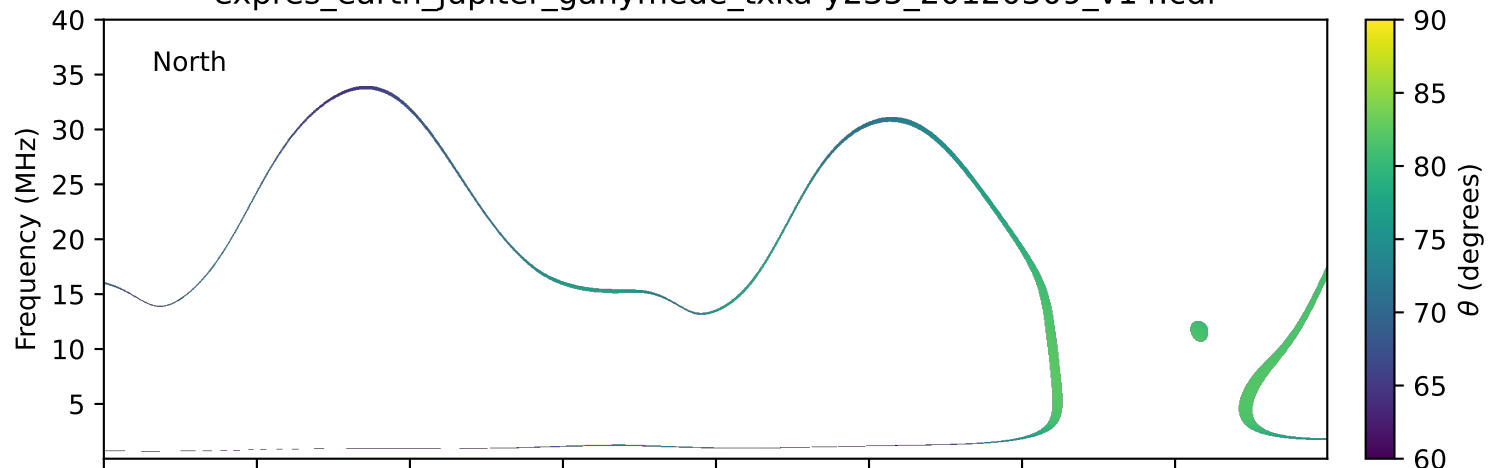
expres_earth_jupiter_ganymede_txka-y235_20120309_v14.cdf
