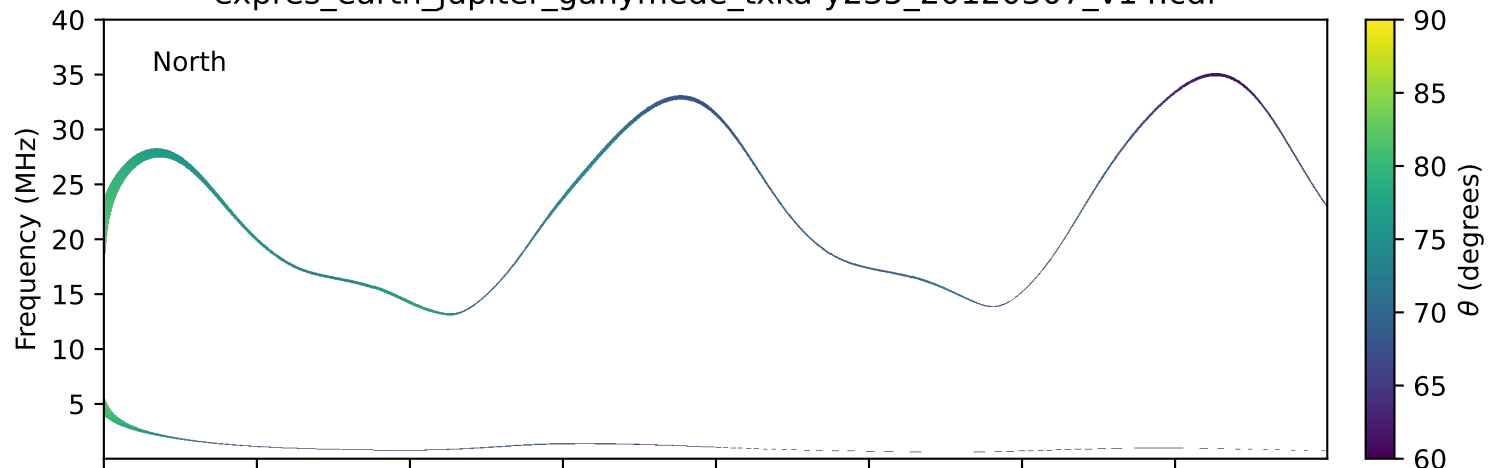
expres_earth_jupiter_ganymede_txka-y235_20120307_v14.cdf
