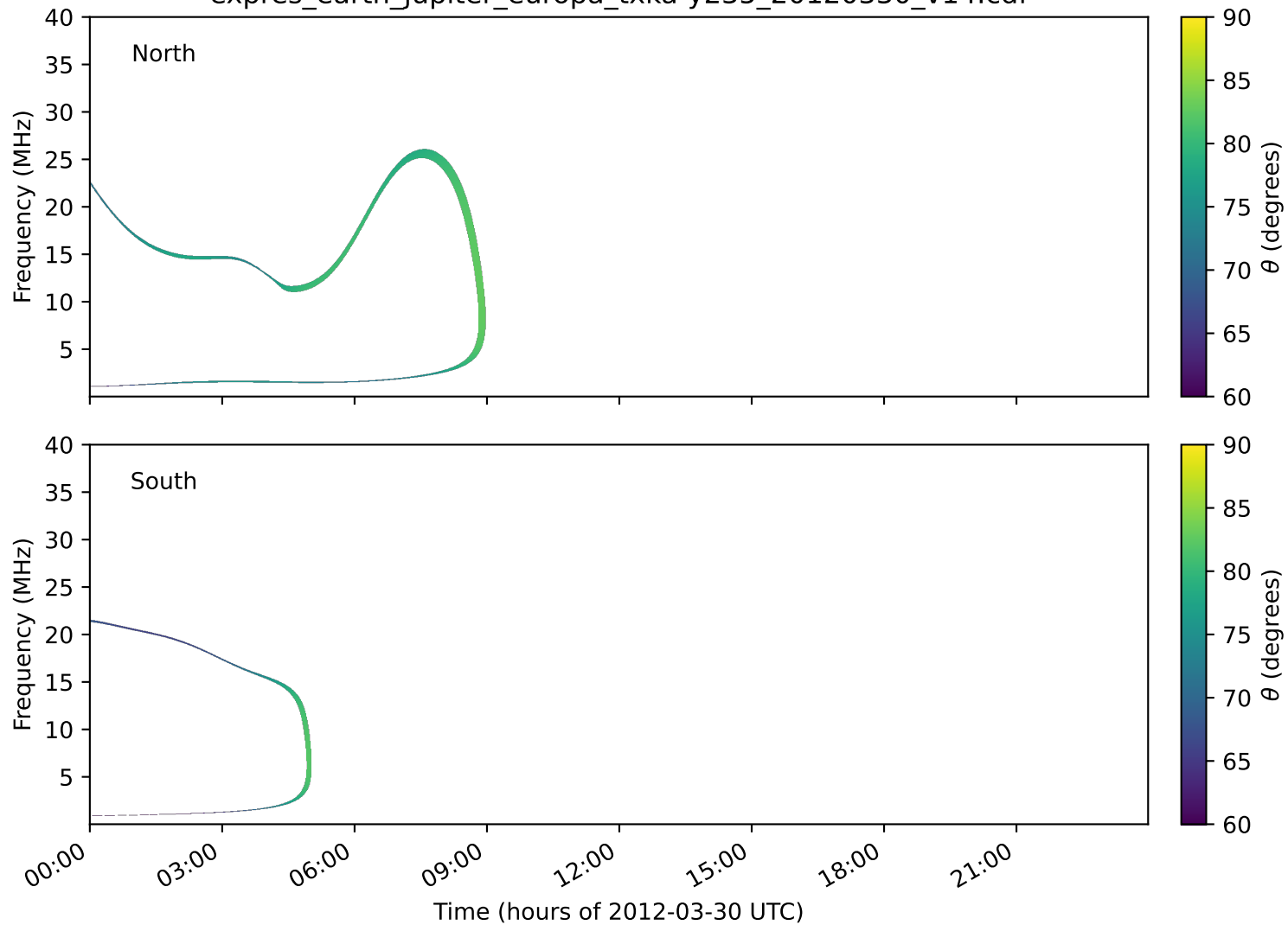
expres_earth_jupiter_europa_txka-y235_20120330_v14.cdf
