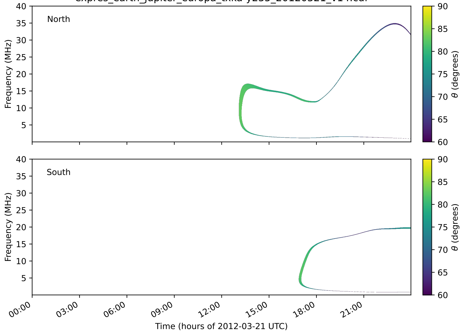
expres_earth_jupiter_europa_txka-y235_20120321_v14.cdf
