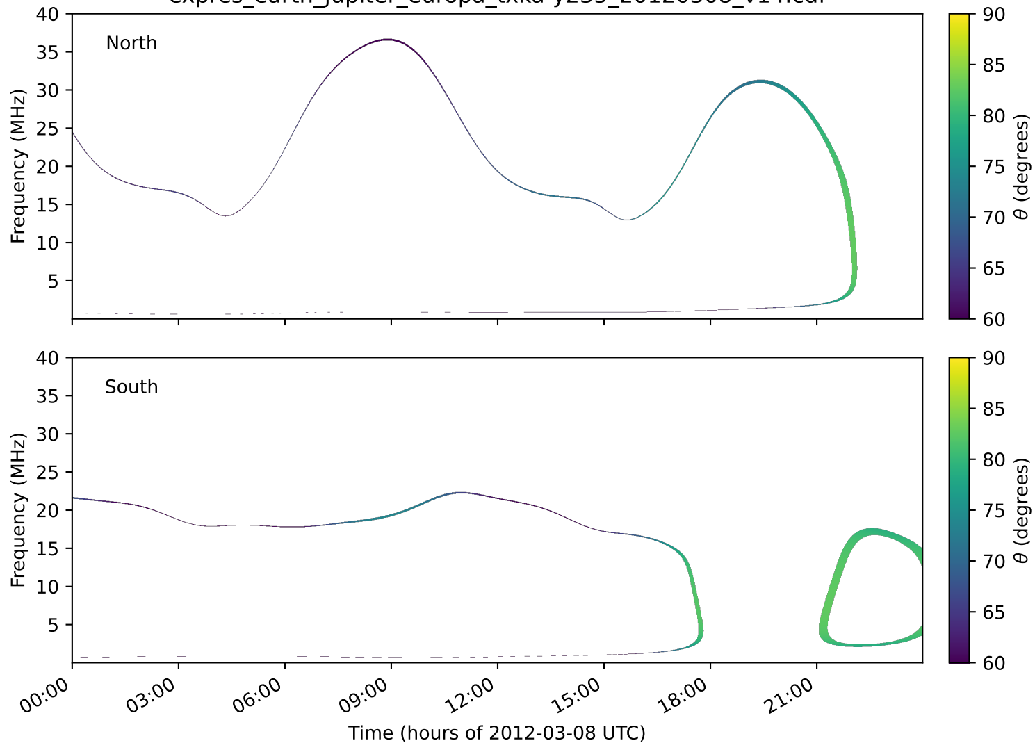
expres_earth_jupiter_europa_txka-y235_20120308_v14.cdf
