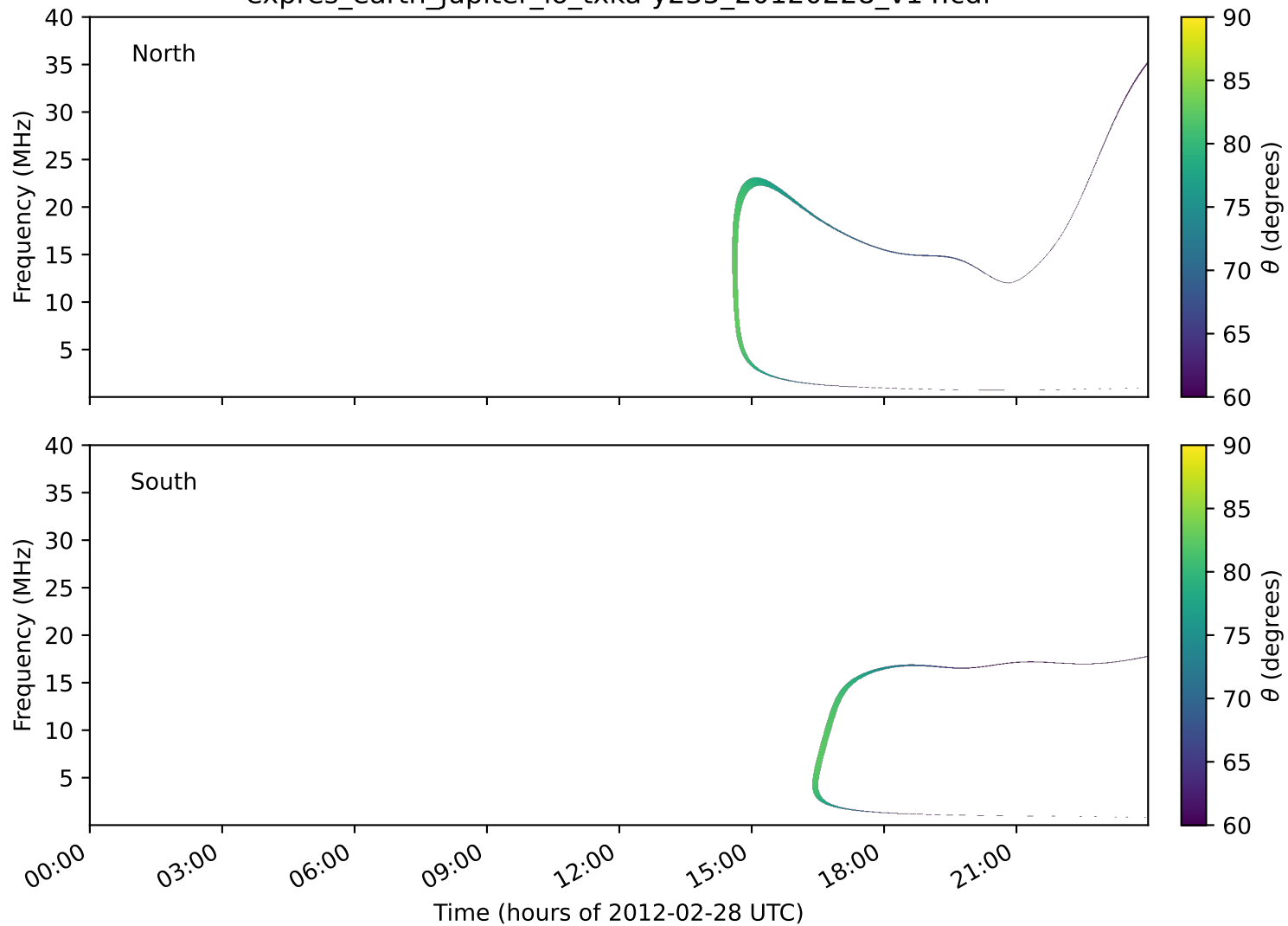
expres_earth_jupiter_io_txka-y235_20120228_v14.cdf
