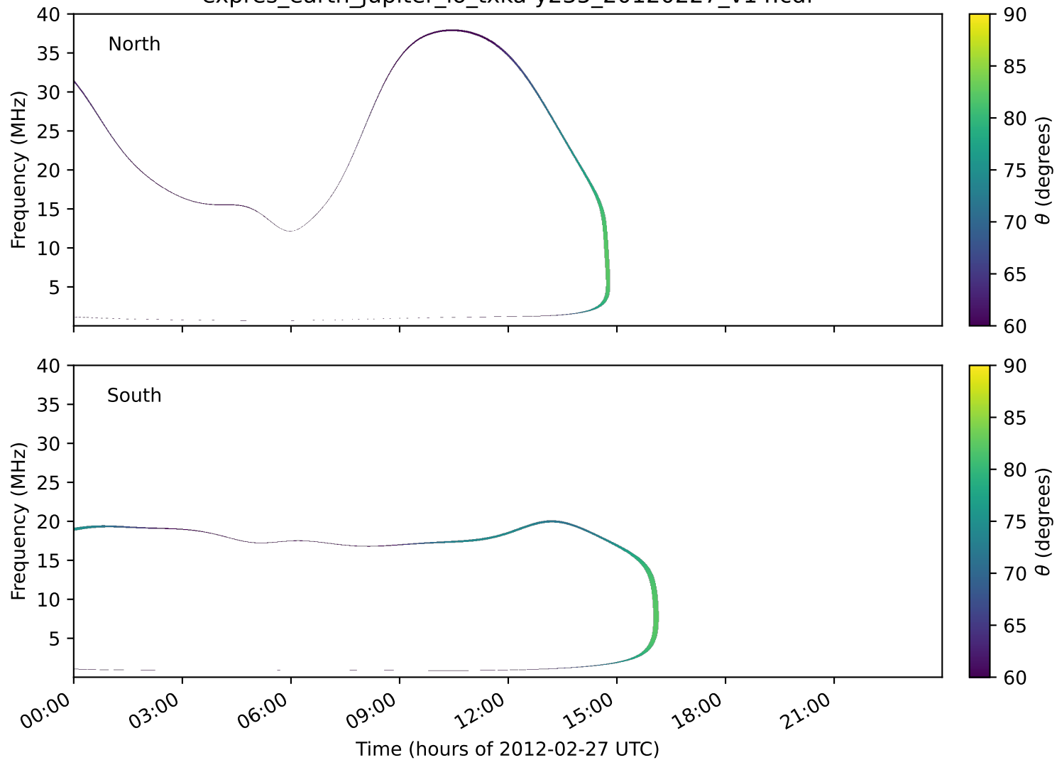
expres_earth_jupiter_io_txka-y235_20120227_v14.cdf
