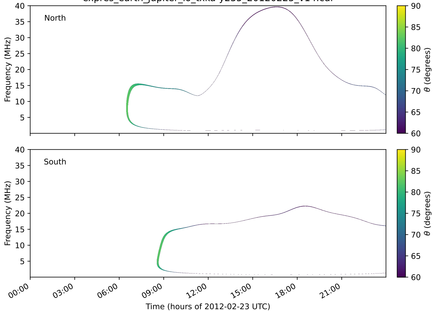
expres_earth_jupiter_io_txka-y235_20120223_v14.cdf
