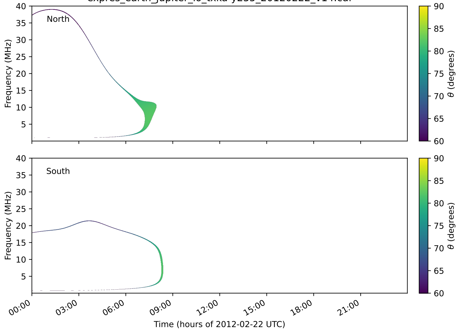
expres_earth_jupiter_io_txka-y235_20120222_v14.cdf
