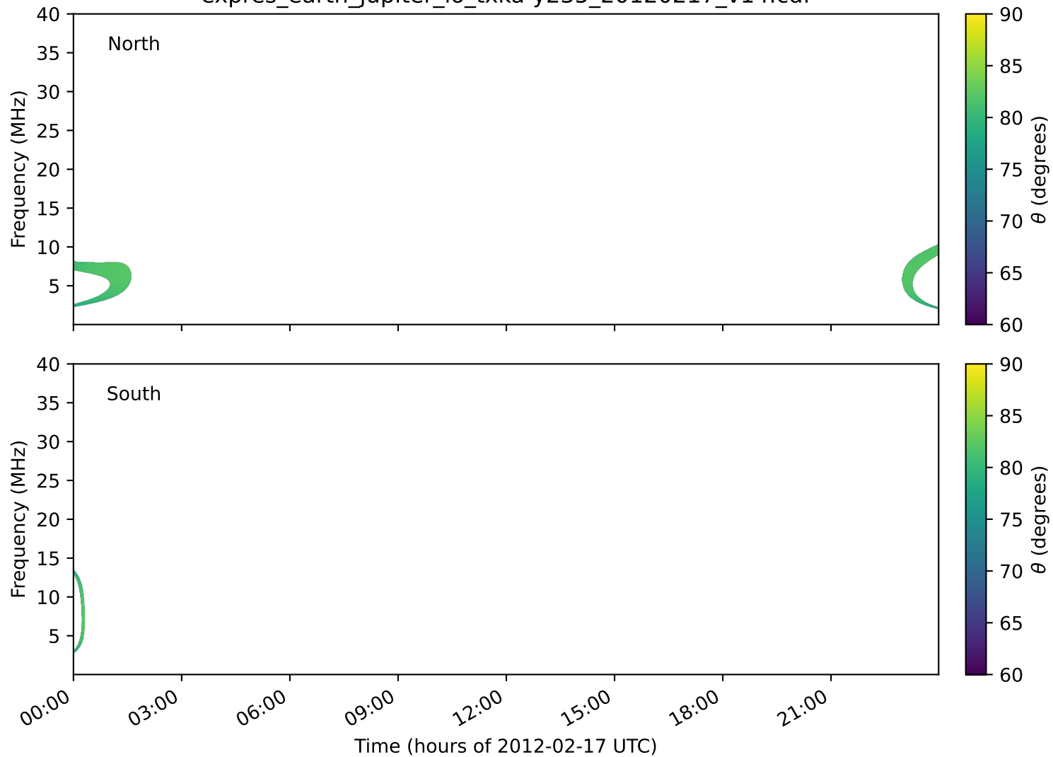
expres_earth_jupiter_io_txka-y235_20120217_v14.cdf
