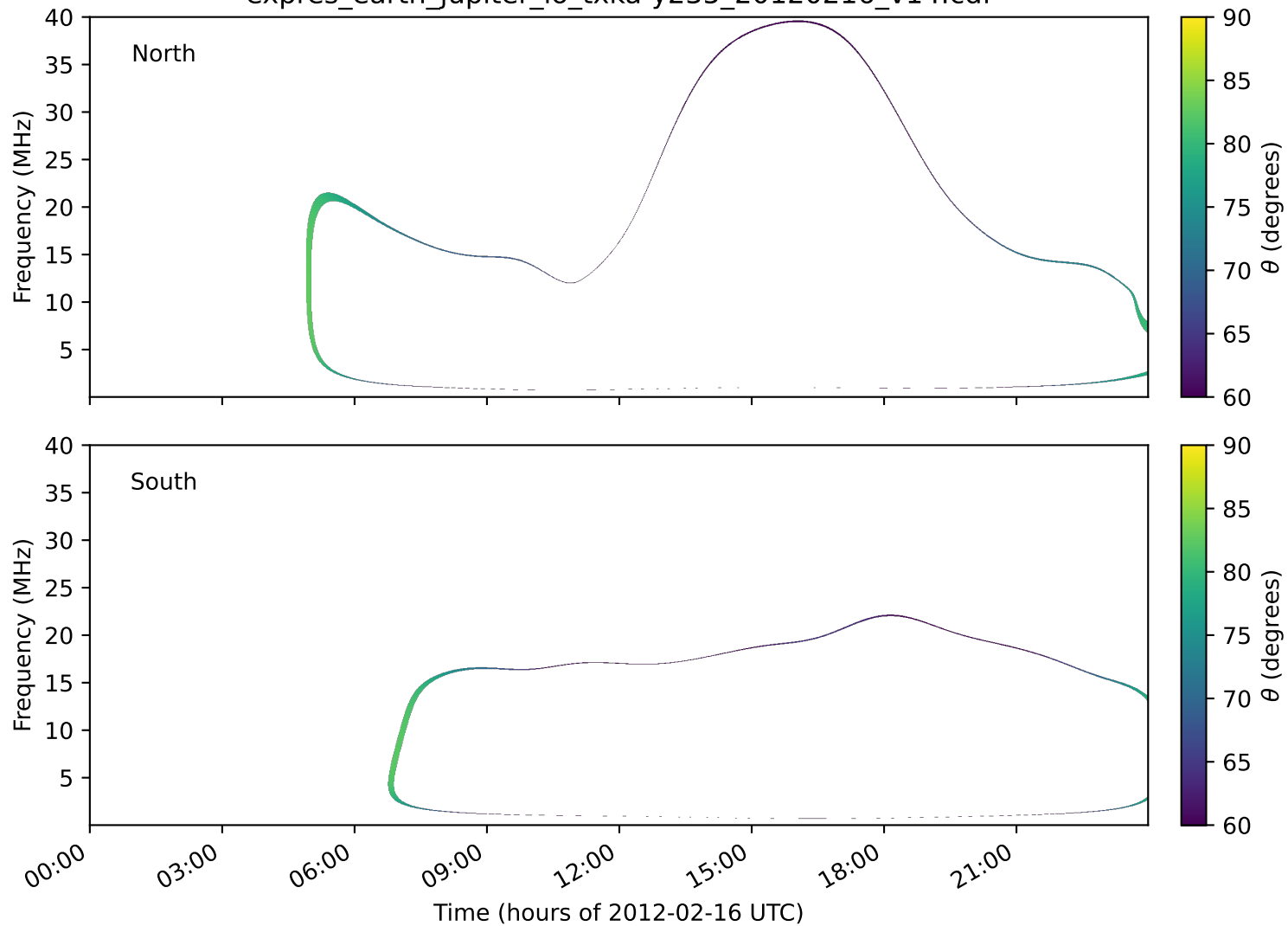
expres_earth_jupiter_io_txka-y235_20120216_v14.cdf
