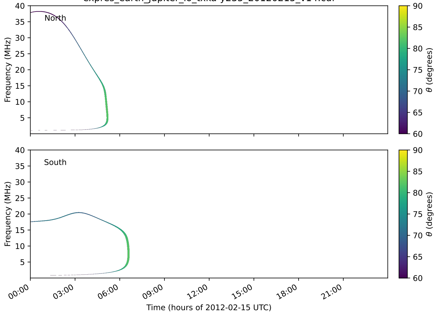
expres_earth_jupiter_io_txka-y235_20120215_v14.cdf
