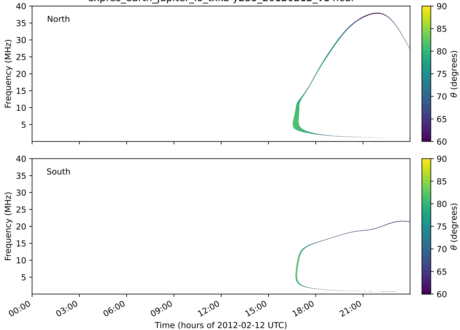
expres_earth_jupiter_io_txka-y235_20120212_v14.cdf
