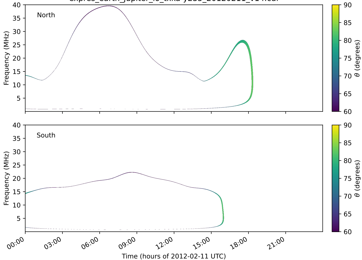
expres_earth_jupiter_io_txka-y235_20120211_v14.cdf
