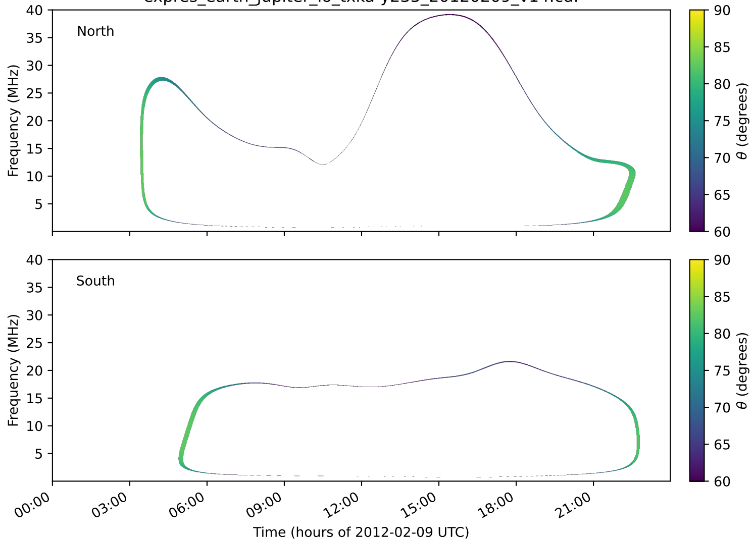
expres_earth_jupiter_io_txka-y235_20120209_v14.cdf
