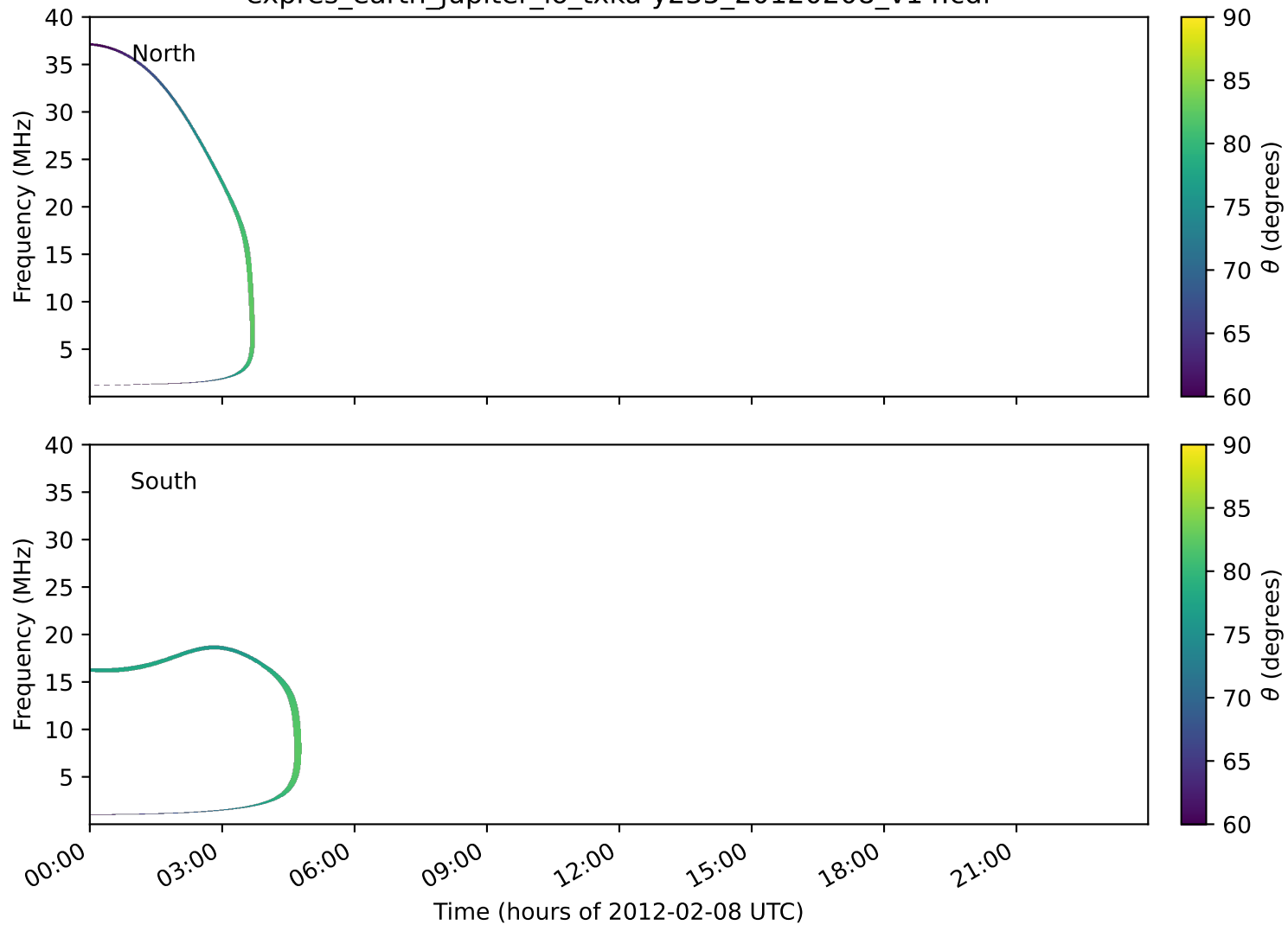
expres_earth_jupiter_io_txka-y235_20120208_v14.cdf
