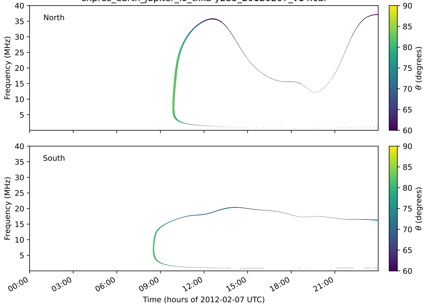
expres_earth_jupiter_io_txka-y235_20120207_v14.cdf
