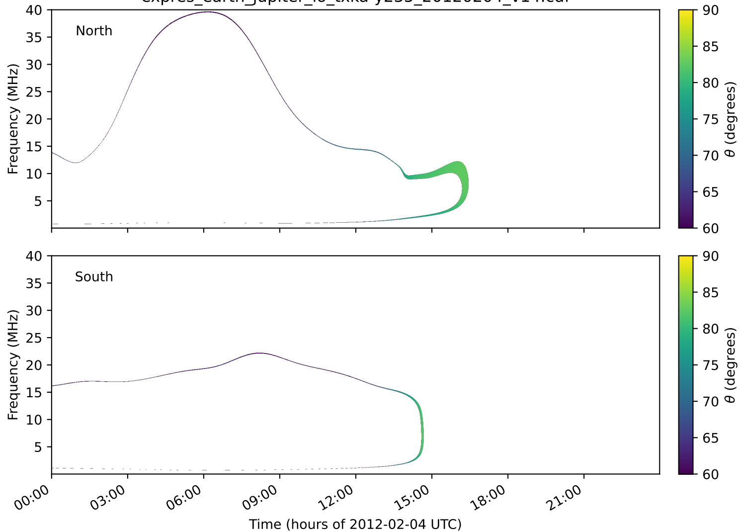
expres_earth_jupiter_io_txka-y235_20120204_v14.cdf
