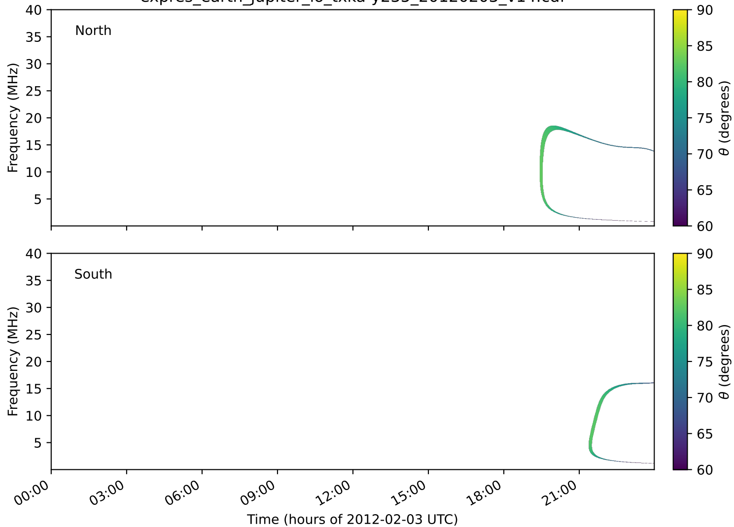
expres_earth_jupiter_io_txka-y235_20120203_v14.cdf
