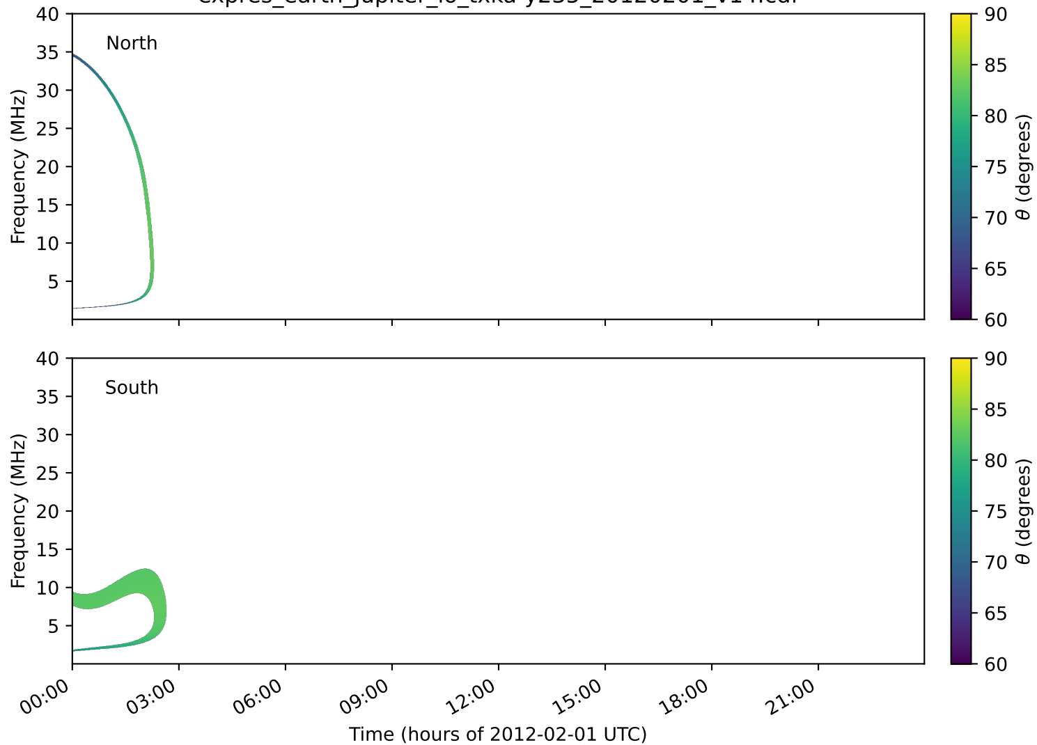
expres_earth_jupiter_io_txka-y235_20120201_v14.cdf
