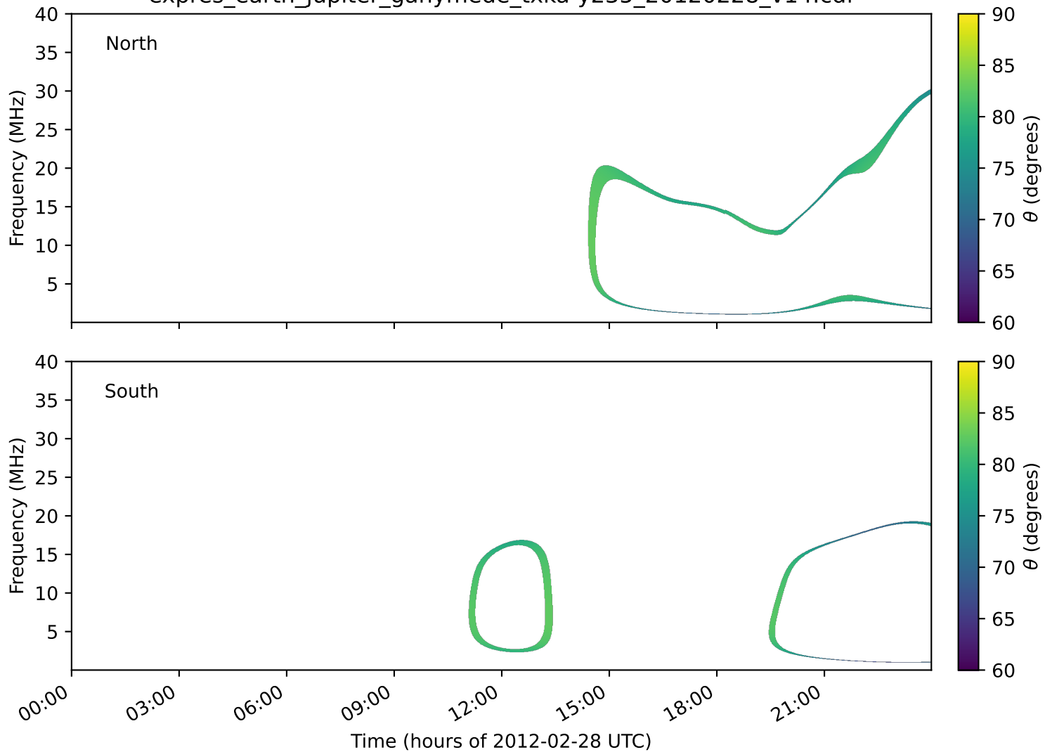
expres_earth_jupiter_ganymede_txka-y235_20120228_v14.cdf
